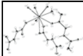
Fig. 1. View of the local coordination of praseodymium(III) with the atom-numbering scheme. Displacement ellipsoids are drawn at the 50% probability level. [Symmetry codes: (i) x, 1/2 - y, -1/2 + z ; (ii) 1 + x, y, z ; (iii) 1 + x, 1/2 - y, -1/2 + z ; (iv) 1 - x, -y, 1 - z ; (v) 2 - x, -y, 1 - z .]
